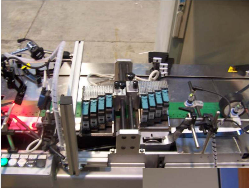
2 x 4 pens on verification system
