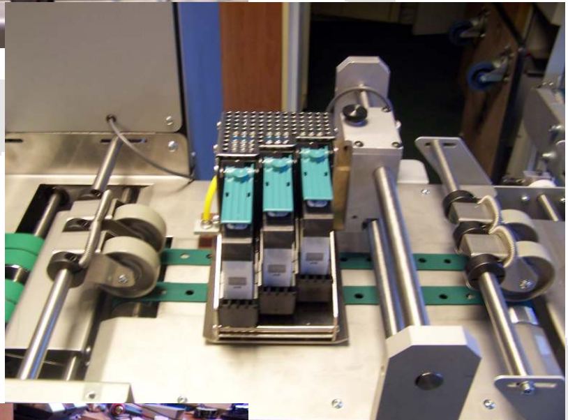
3 pen stall on rejector
